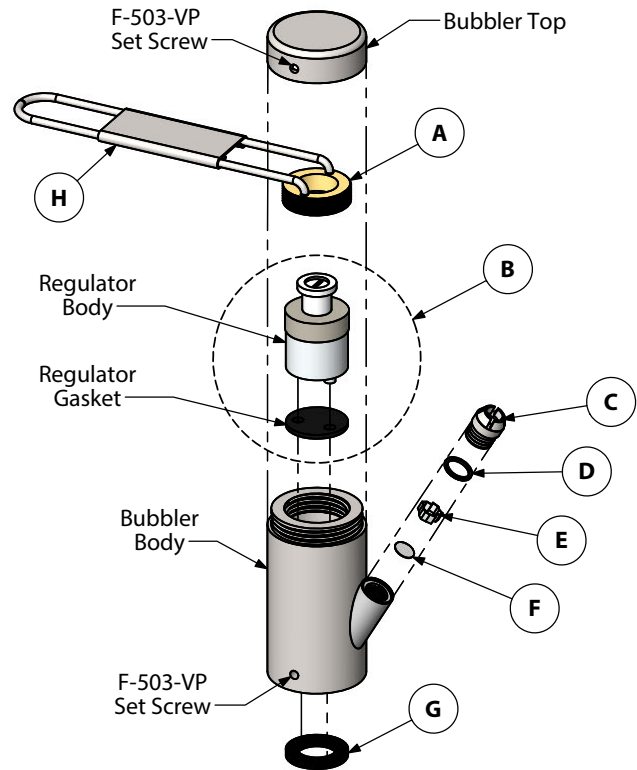
Exploded View F-503 Bubbler Assembly
