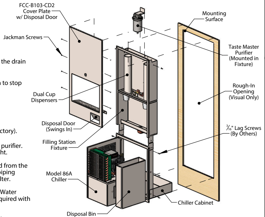
FCC-B103-CD2 Models Include Taste Master Purifier with Three Elements
