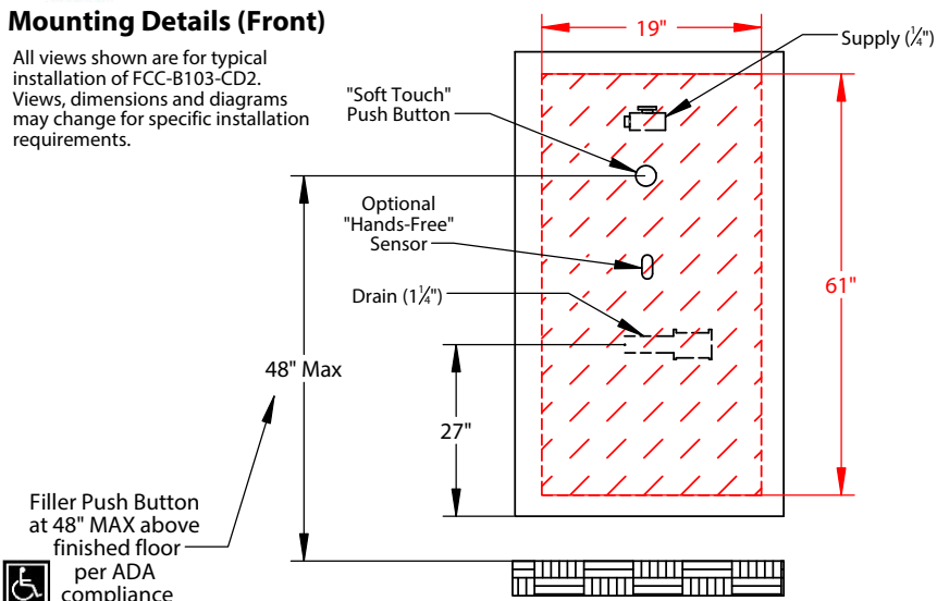
FCC-B103-CD2 Models Include 86A Chiller
